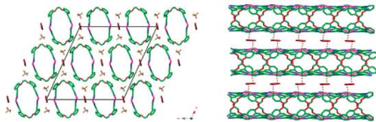
Figure 4. The packing of the tubes in 4 (left). Also shown are the \text{BF}_4^- counterions and the bis- \eta^1 -coordinated benzene molecules. One layer (right) defined by the weak intermolecular \text{Ag}\cdots\pi interactions between the tubes and the intercalated benzene molecules (highlighted in brown).
